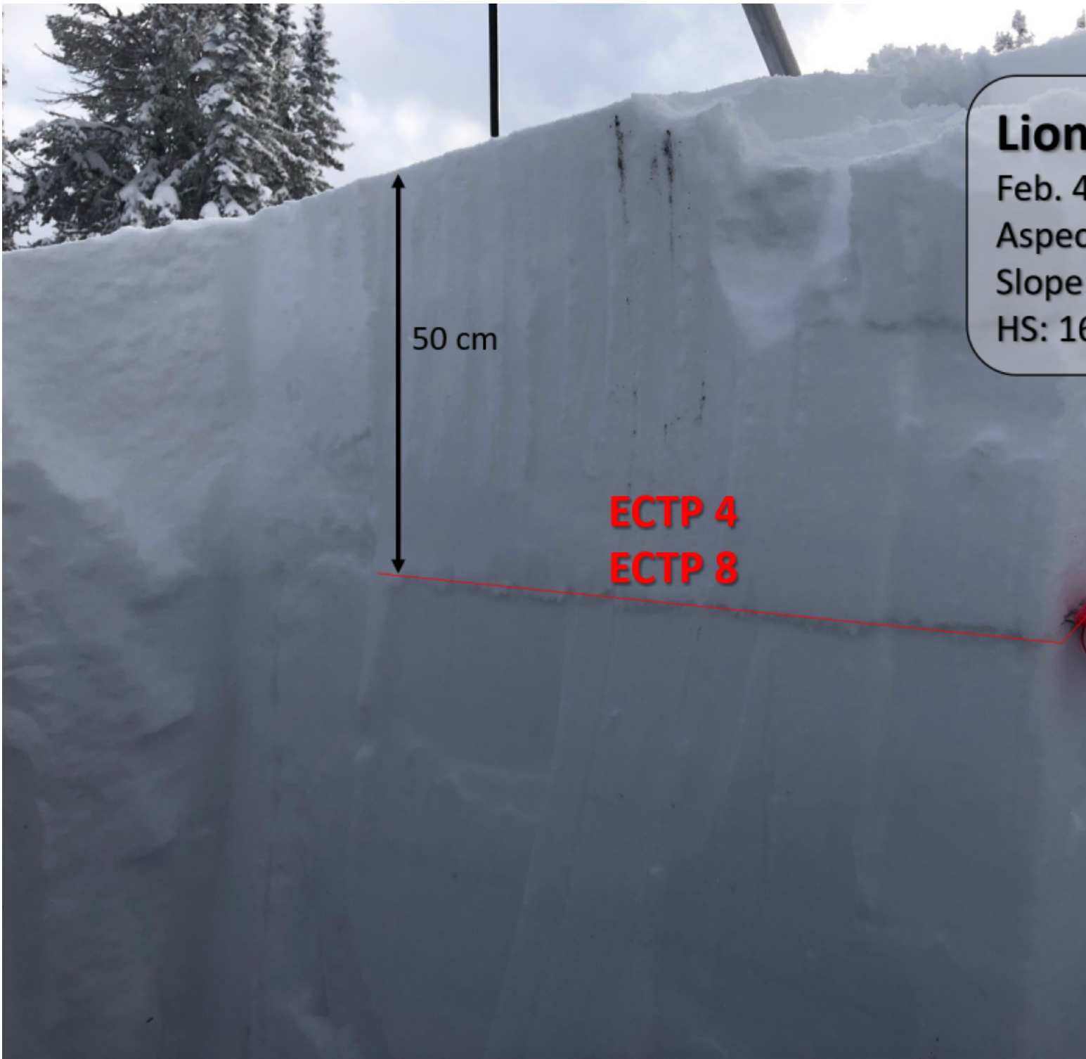
Snowmobilers in the Lionhead area got unstable test results, easily propagating fractures in ECT tests on a weak layer buried about 50 cm deep. Photo: J. Norlander
